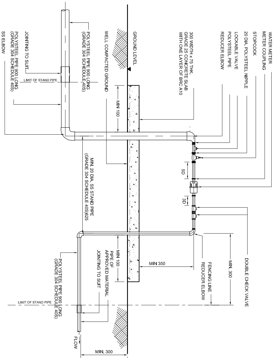
TYPICAL DETAILS OF POLYSTEEL METER STAND INSTALLATION FOR SINGLE METER SIZE 15 - 50 DIA. ~ TYPE A
